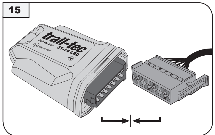
Modul Trail-tec 31-14 LED → Stecker 14 pin E-Satz modul Trail-tec 31-14 LED → socket 14 pin e-kit
